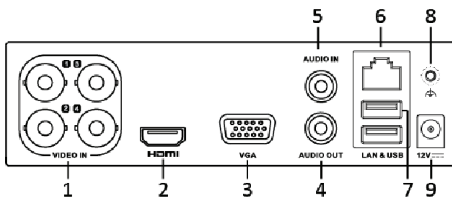
Rear Panel of MZ 40MTS
