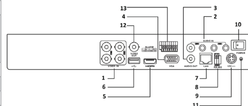
Rear Panel of MZ 40HT
