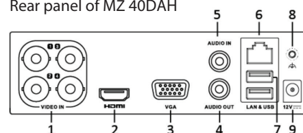
Rear panel of MZ 40DAH
